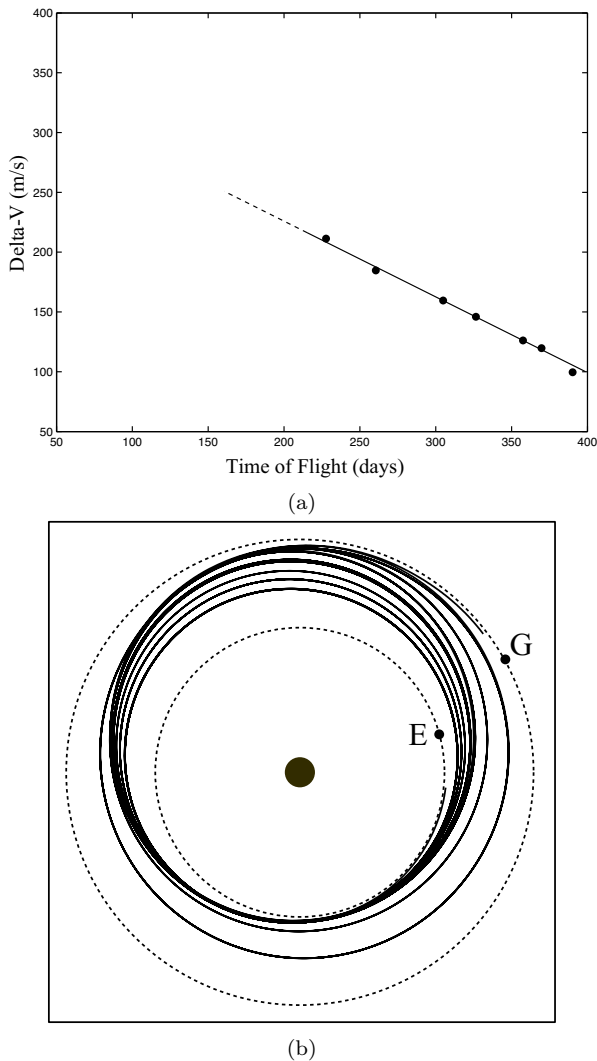
FIGURE 10.4.2. Fuel consumption versus flight time trade-off for the inter-moon transfer phase of a multi-moon orbiter mission. (a) The \Delta V vs. time of flight plot for several transfer trajectories from Ganymede to Europa are shown. For the several cases run, we find a near linear relationship between \Delta V and time of flight. For this study we looked at a range of energies in both three-body systems. The highest energy (and lowest TOF) transfer we computed is shown in (b) in inertial coordinates, where G labels Ganymede's orbit and E labels Europa's. This transfer has a TOF of 227 days and a \Delta V of 211 m/s. Beyond this lower TOF limit to the computations, we speculate that the linearity will continue for a while, indicated by the dashed line.
