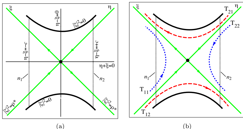
FIGURE 2.7.1. The projection onto the \eta - \xi plane of orbits near the equilibrium point (note, axes tilted 45°). (a) The equilibrium region, \mathcal{R} , is bounded by the thick hyperbolic segments at top and bottom and the dotted vertical segments at left and right. At the origin is the periodic orbit in \mathcal{R} . The thick lines with arrows pointing toward or away from the origin are trajectories asymptotically winding onto the periodic orbit. See the text for further descriptions. (b) Four additional trajectories are shown. The labeling T_{ij} denotes the path of a particle which entered \mathcal{R} through n_i and exited through n_j . Two transit orbits, T_{12} and T_{21} , and two non-transit orbits, T_{11} and T_{22} , are shown.
