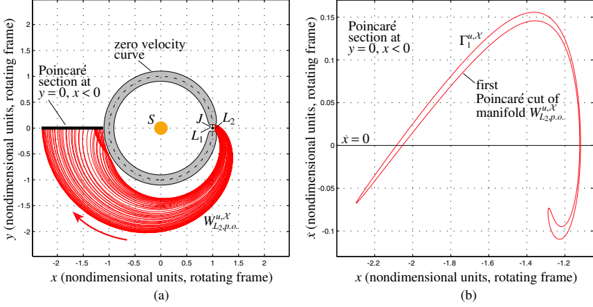
FIGURE 3.4.1. (a) The position space projection of the unstable manifold “tube” W_{L2,p.o.}^{u,\mathcal{X}} until the first intersection with the Poincaré section at y = 0, x < 0 . (b) The first Poincaré cut \Gamma_1^{u,\mathcal{X}} of the manifold W_{L2,p.o.}^{u,\mathcal{X}} on the plane y = 0, x < 0 .
