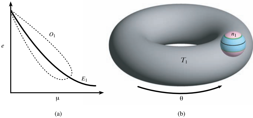
FIGURE 3.2.3. (a) Open set O_1 in (\mu, e) -plane. (b) The region T_1 with meridional angular coordinate \theta .
