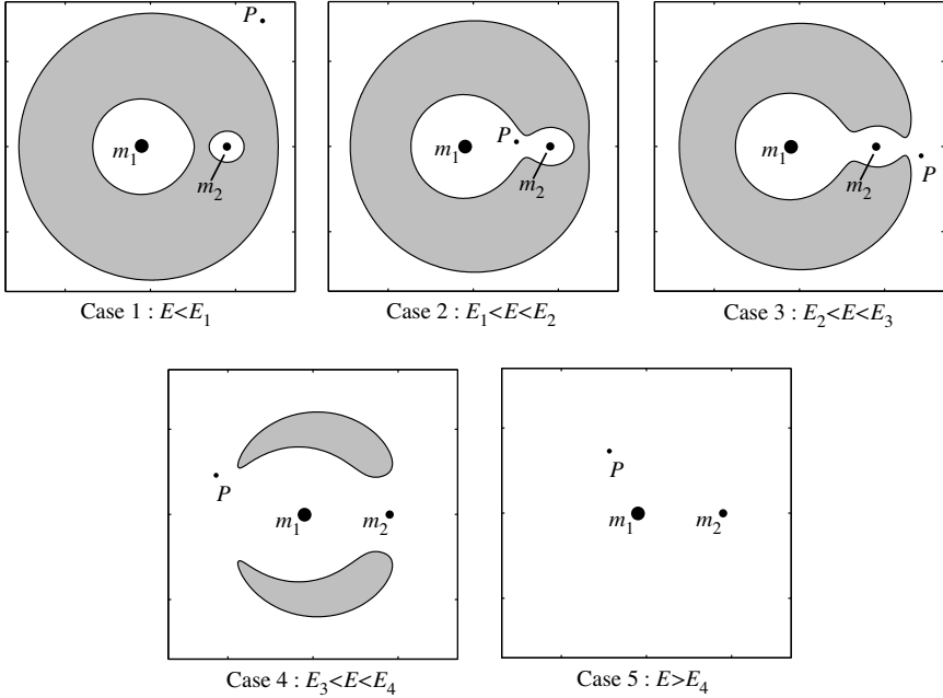
FIGURE 2.4.2. Realms of possible motion. Zero velocity curves for five values of the energy, one in each of the cases as described in the text, are shown on the x-y plane for \mu = 0.3 . These curves bound the zone, in white, accessible by the particle, P , for a given energy value, E = e . The part of the x-y plane which is shaded is inaccessible for a given energy, and known as the forbidden realm . The outermost accessible realm, known as the exterior realm , extends to infinity. In the fifth case (e), the forbidden realm vanishes and motion over the entire x-y plane is possible.
