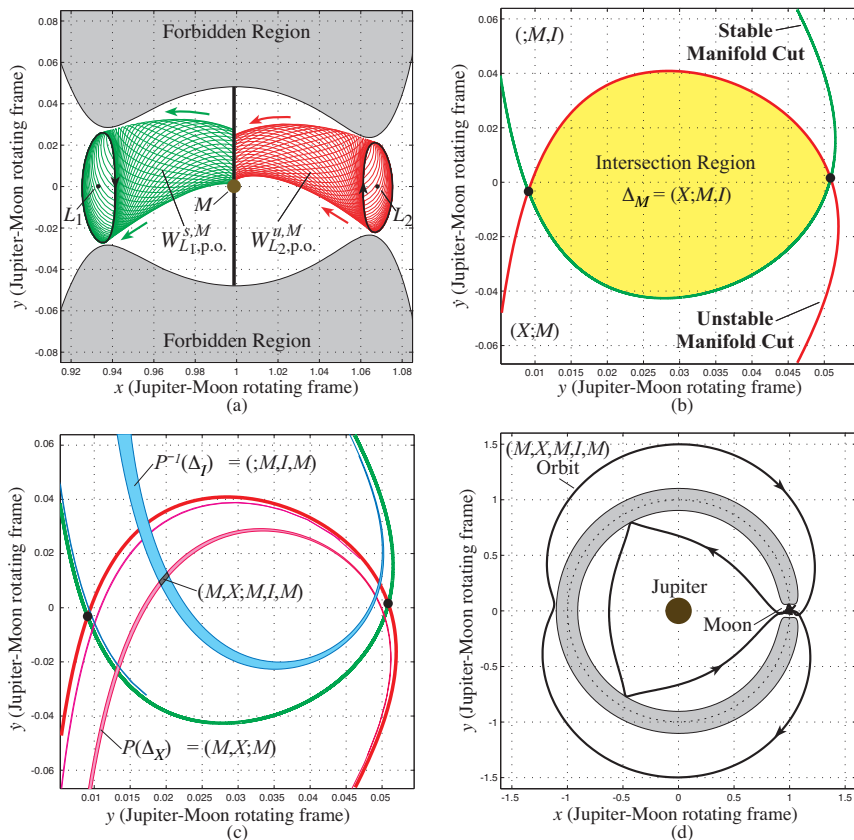
FIGURE 9.4.2. (a) The projection of invariant manifolds W_{L1,p.o.}^{s,M} and W_{L2,p.o.}^{u,M} in the realm M of the position space. (b) A close-up of the intersection region between the Poincaré cuts of the invariant manifolds on the U_3 section ( x = 1 - \mu, y > 0 ). (c) Intersection between image of \Delta_X and pre-image of \Delta_I labeled (M, X; M, I, M) . (d) Example orbit passing through (M, X; M, I, M) region of (c).
