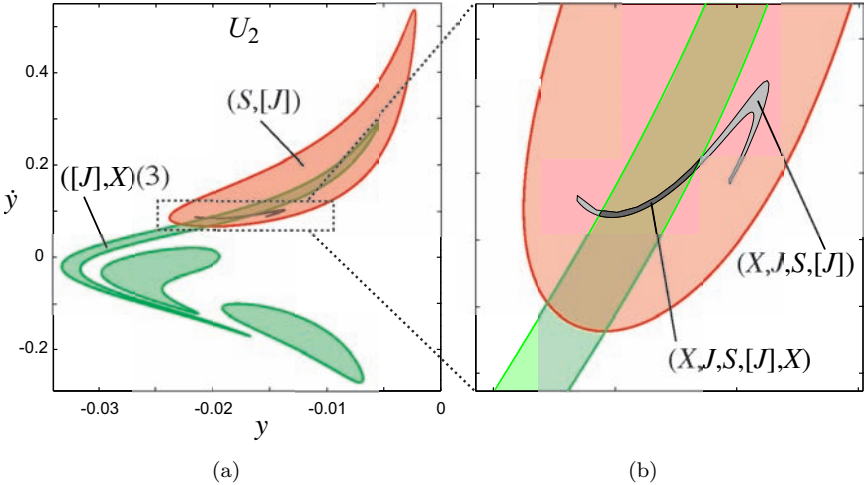
FIGURE 4.5.3. (a) We evolve the larger of the (X, J, [S], J) pieces on U_1 until it intersects U_2 . (b) A close-up of the intersection of the (X, J, S, [J]) and ([J], X) itinerary regions is shown, yielding the desired (X, J, S, [J], X) region.
