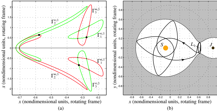
FIGURE 3.4.4. (a) The first three Poincaré cuts of the unstable ( W_{L_1, \text{p.o.}}^{u, \mathcal{S}} ) and stable ( W_{L_1, \text{p.o.}}^{s, \mathcal{S}} ) manifolds with the plane y = 0 . (b) A nonsymmetric (1, 3) -homoclinic orbit in the interior realm (corresponding to the three large dots in (a)).
