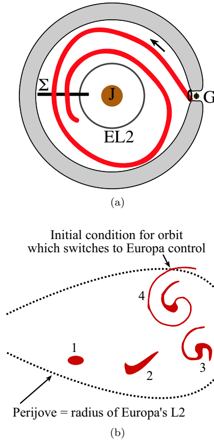
FIGURE 10.4.1. Numerical construction of natural trajectory arcs which will switch control from Ganymede to Europa. Suppose we want to find trajectories which begin near Ganymede (G in the figure) and escape toward Europa, finally getting naturally captured by Europa. The first step is to numerically construct the Ganymede L_1 tube heading toward Europa, or U(\text{Ga}_{L1}) in the terminology of the text. We take a Poincaré section, \Sigma , at the position shown in (a). We show only two crossings of \Sigma , but there are an infinite number. We also show the radial distance of Europa's L_2 , labeled EL2, and the forbidden region at this energy. In (b), we show a schematic of the initial cross-section of the tube on \Sigma , labeled 1. The successive crossings are labeled 2, 3, .... In this schematic, we also show the dotted line corresponding to a perijove equal to the radial distance of Europa's L_2 . The first three crossings are entirely within the zone of perijoves greater than the radial distance of Europa's L_2 . Any spacecraft trajectory in the Jupiter-Ganymede-spacecraft system which crosses this line can be assumed to “switch” control to Europa, meaning the Jupiter-Europa-spacecraft system becomes a good approximation from then on. The coordinates represented here are not quasi-action-angle coordinates as in Figures 10.3.1 and 10.2.2(a), but are related to cartesian coordinates, which are easier to handle numerically.
