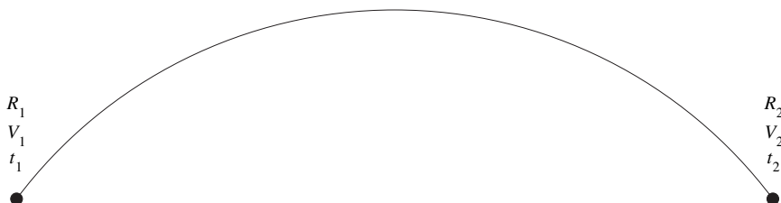
FIGURE 7.5.1. Level I Differential Corrector: two patch points.
