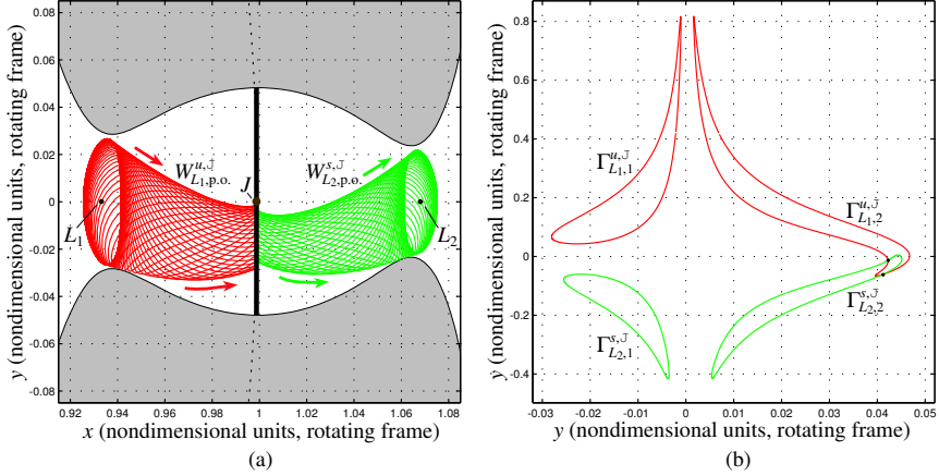
FIGURE 3.5.1. (a) The projection of invariant manifolds W_{L_1, \text{p.o.}}^{u, \mathcal{J}} and W_{L_2, \text{p.o.}}^{s, \mathcal{J}} in the realm \mathcal{J} of the position space. (b) The first two Poincaré cuts of the invariant manifolds with the plane x = 1 - \mu .
