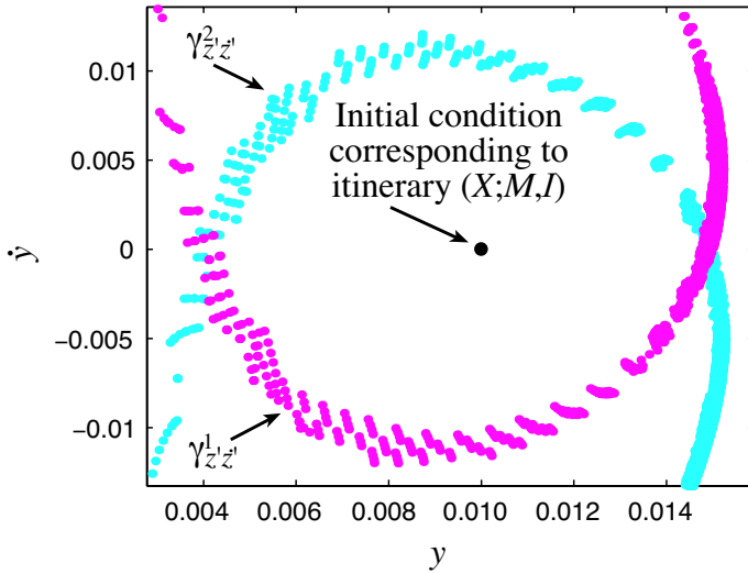
FIGURE 9.4.5. On the (y, \dot{y}) -plane are shown the points that approximate \gamma_{z',z'}^2 and \gamma_{z',z'}^1 , the boundaries of \text{int}(\gamma_{z',z'}^2) and \text{int}(\gamma_{z',z'}^1) , respectively, where (z', \dot{z}') = (0.0035, 0) . Note the lemon shaped region of intersection, \text{int}(\gamma_{z',z'}^1) \cap \text{int}(\gamma_{z',z'}^2) , in which all orbits have the itinerary (X; M, I) . The appearance is similar to Figure 9.4.2(b). The point shown within \text{int}(\gamma_{z',z'}^1) \cap \text{int}(\gamma_{z',z'}^2) is the initial condition for the orbit shown in Figure 9.4.6.
