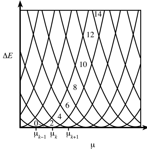
FIGURE 3.3.2. Partition of the (\mu, \Delta E) -plane according to the number of symmetric (1,1)-homoclinic points found in the first intersection of W_{L_1, \text{p.o.}}^{u,S} with the plane y = 0, x < 0 .
