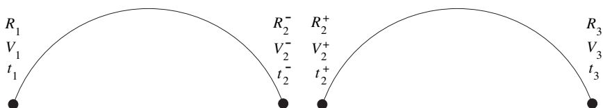
FIGURE 7.5.2. Level II Differential Corrector: 3 patch points.
